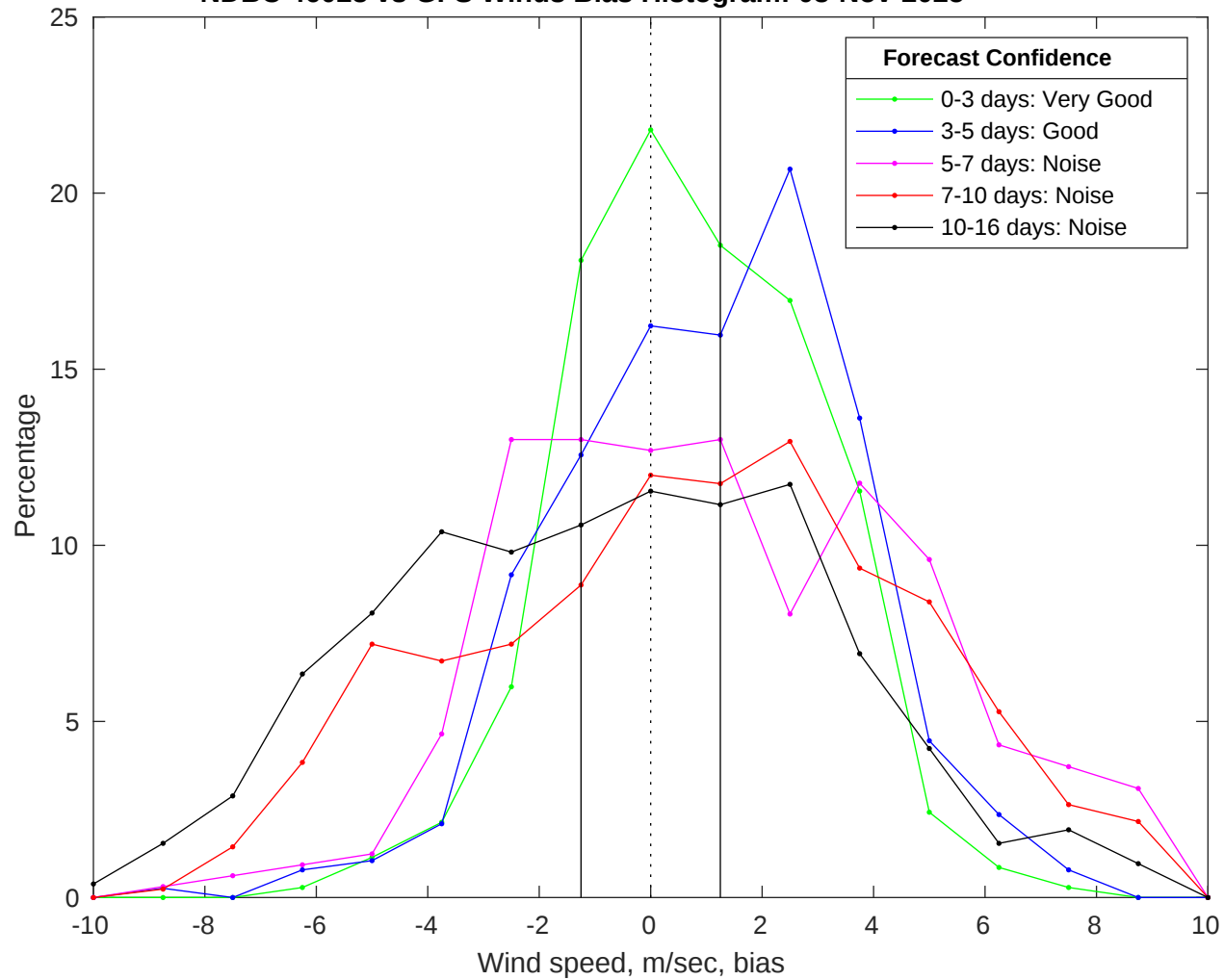
NDBC 46028 vs GFS Winds Bias Histogram: 03-Nov-2025
