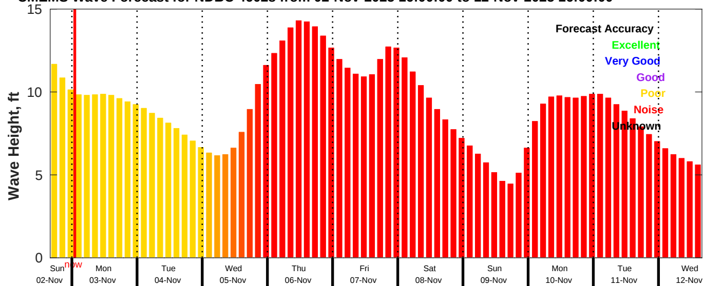
CMEMS Wave Forecast for NDBC 46028 from 02-Nov-2025 16:00:00 to 12-Nov-2025 16:00:00
