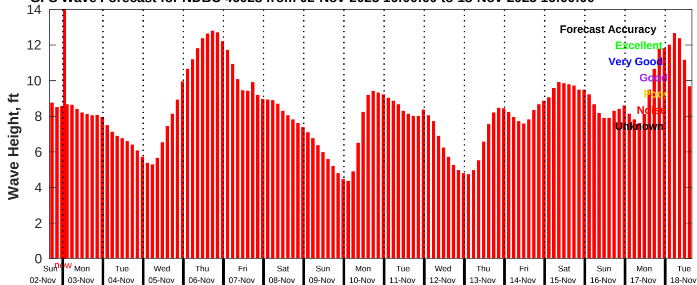
GFS Wave Forecast for NDBC 46028 from 02-Nov-2025 16:00:00 to 18-Nov-2025 16:00:00
