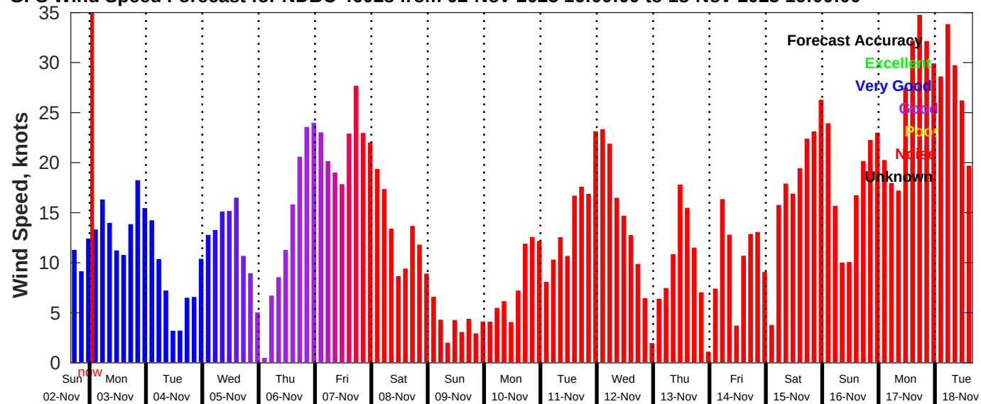
GFS Wind Speed Forecast for NDBC 46028 from 02-Nov-2025 16:00:00 to 18-Nov-2025 16:00:00
