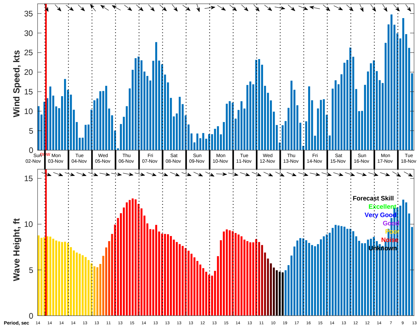
Wind & Wave Forecast for NDBC 46028 from 02-Nov-2025 16:00:00 to 18-Nov-2025 16:00:00
