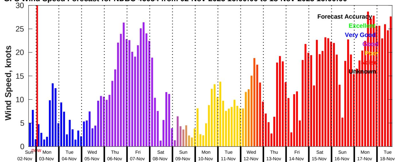
GFS Wind Speed Forecast for NDBC 46054 from 02-Nov-2025 16:00:00 to 18-Nov-2025 16:00:00
