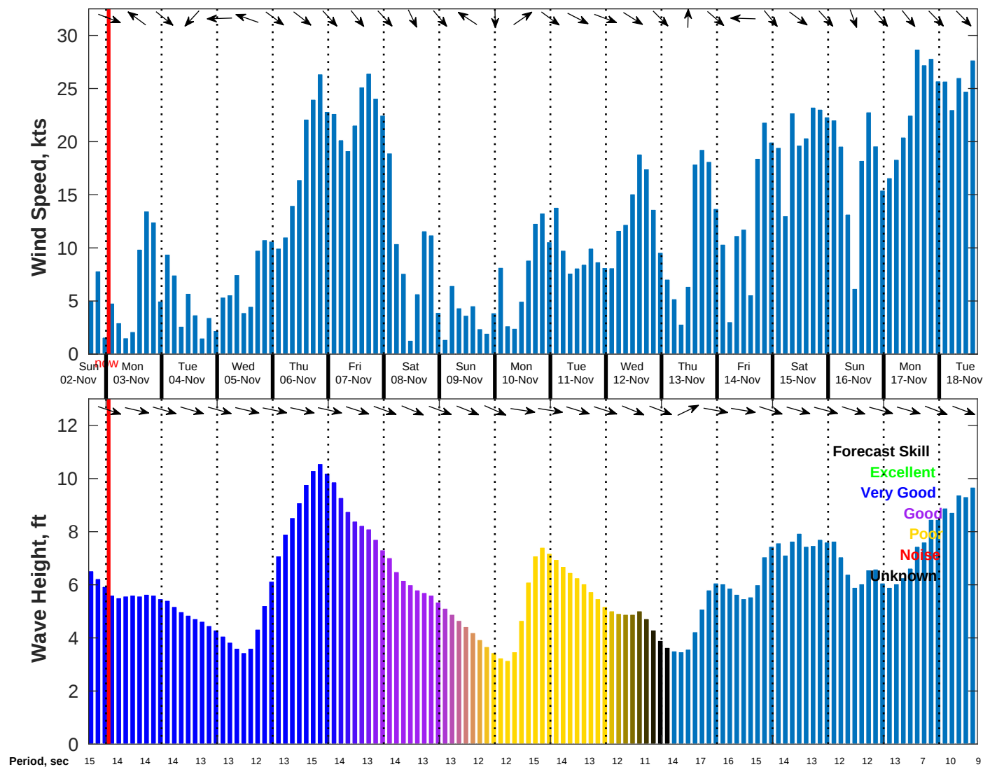
Wind & Wave Forecast for NDBC 46054 from 02-Nov-2025 16:00:00 to 18-Nov-2025 16:00:00
