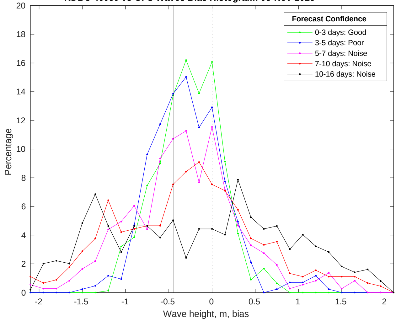
NDBC 46059 vs GFS Waves Bias Histogram: 03-Nov-2025
