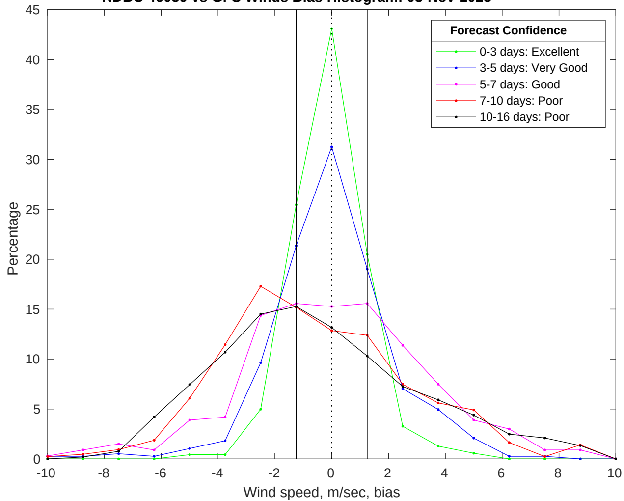
NDBC 46059 vs GFS Winds Bias Histogram: 03-Nov-2025
