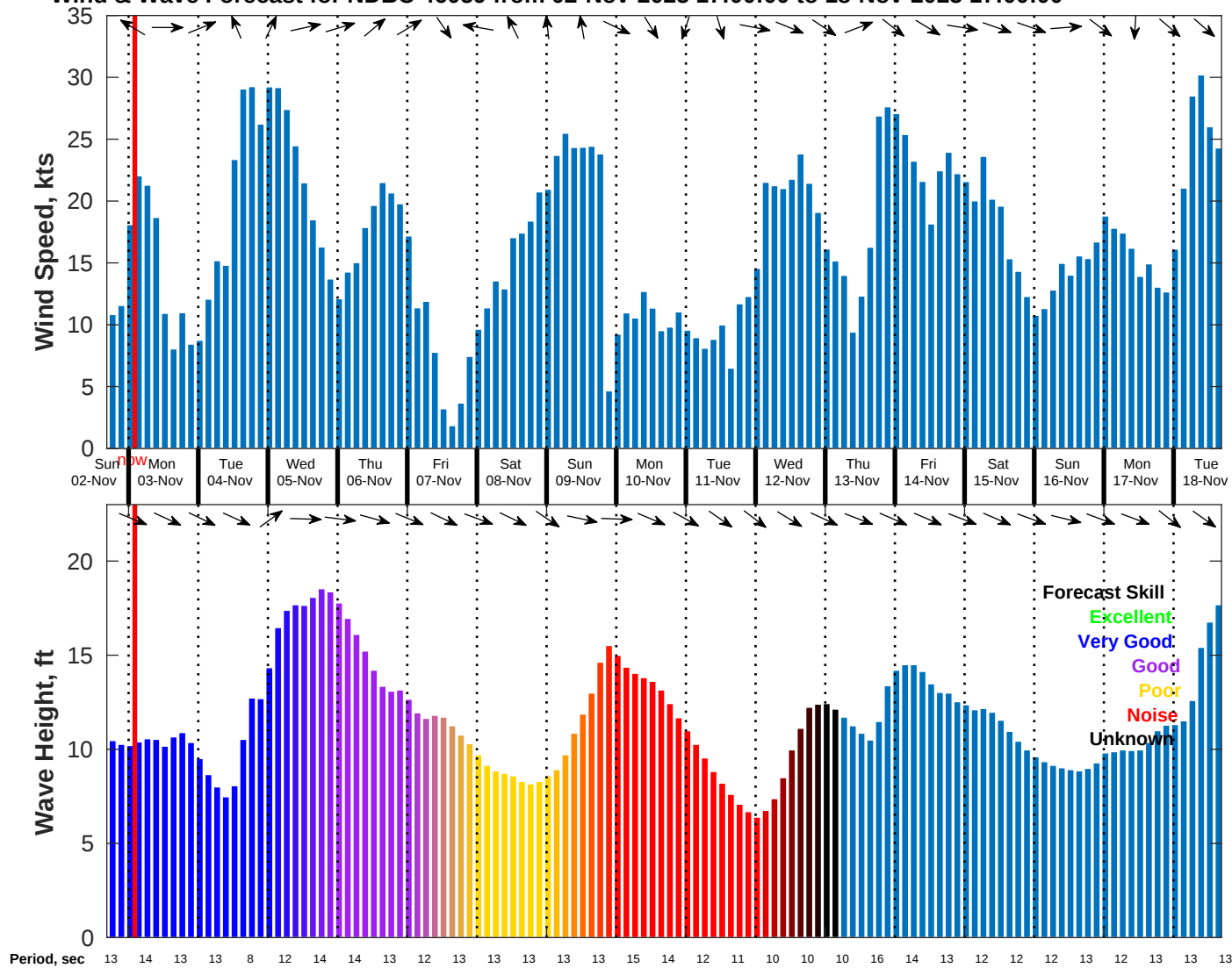
Wind & Wave Forecast for NDBC 46059 from 02-Nov-2025 17:00:00 to 18-Nov-2025 17:00:00
