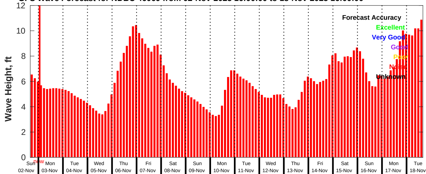
GFS Wave Forecast for NDBC 46069 from 02-Nov-2025 16:00:00 to 18-Nov-2025 16:00:00
