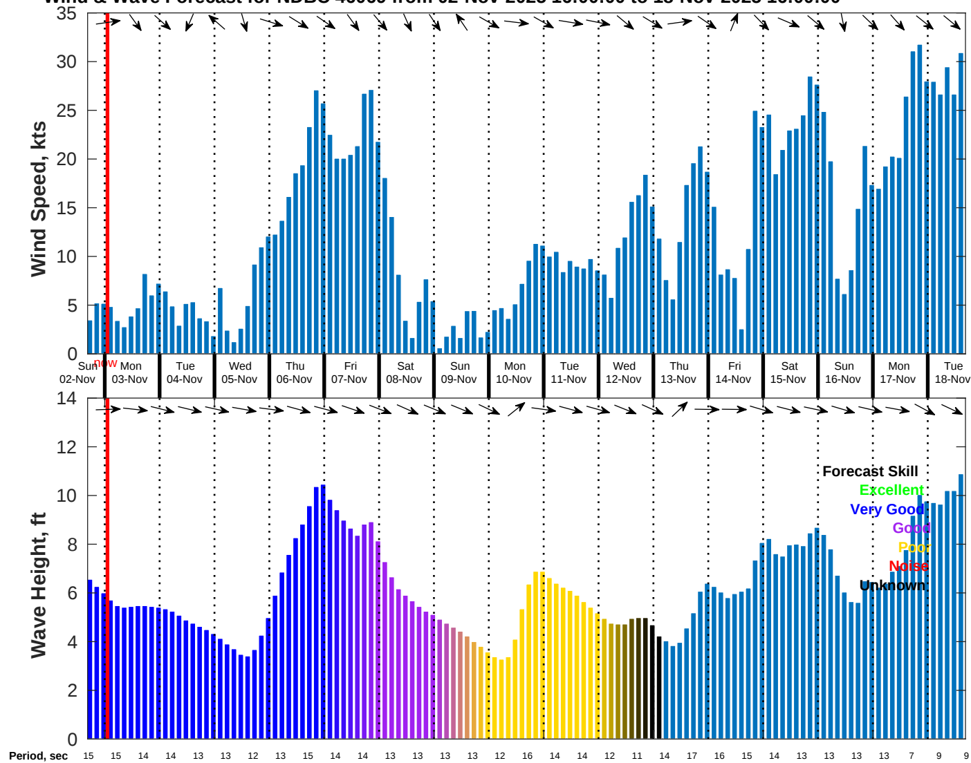
Wind & Wave Forecast for NDBC 46069 from 02-Nov-2025 16:00:00 to 18-Nov-2025 16:00:00
