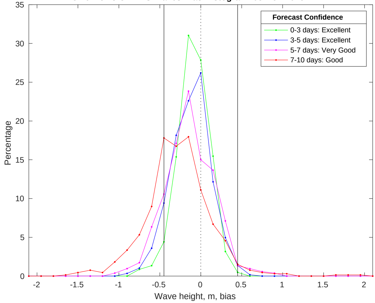
NDBC 46215 vs CMEMS Waves Bias Histogram: 03-Nov-2025
