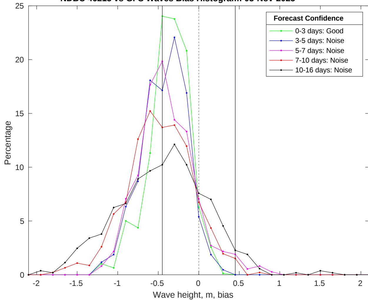
NDBC 46215 vs GFS Waves Bias Histogram: 03-Nov-2025
