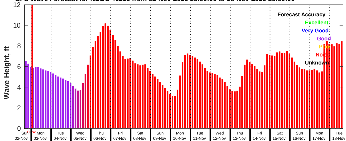
GFS Wave Forecast for NDBC 46215 from 02-Nov-2025 16:00:00 to 18-Nov-2025 16:00:00
