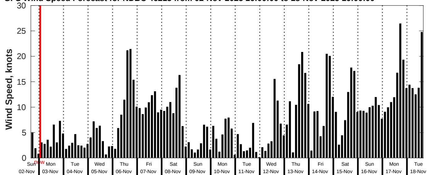
GFS Wind Speed Forecast for NDBC 46215 from 02-Nov-2025 16:00:00 to 18-Nov-2025 16:00:00
