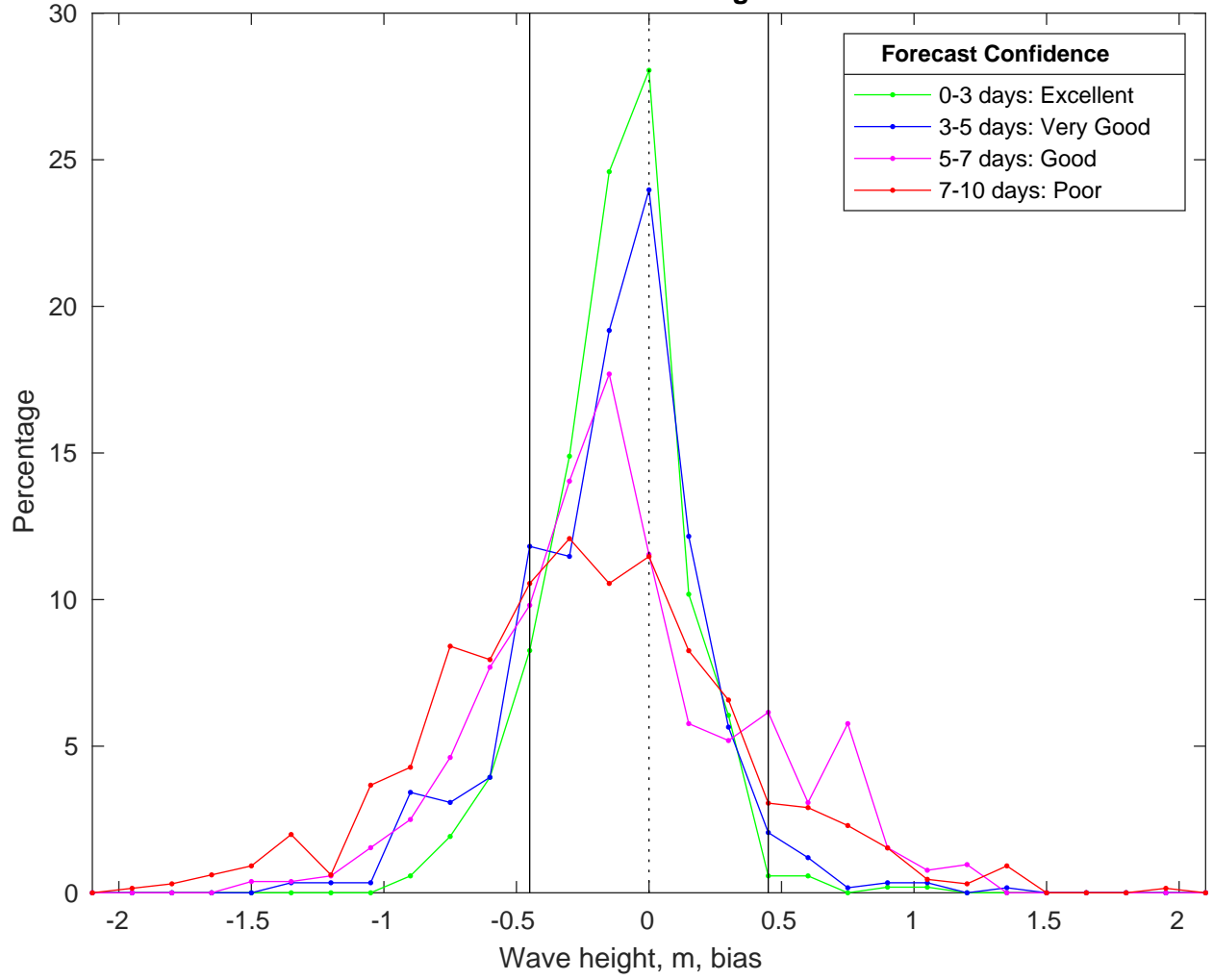
NDBC 46259 vs CMEMS Waves Bias Histogram: 03-Nov-2025
