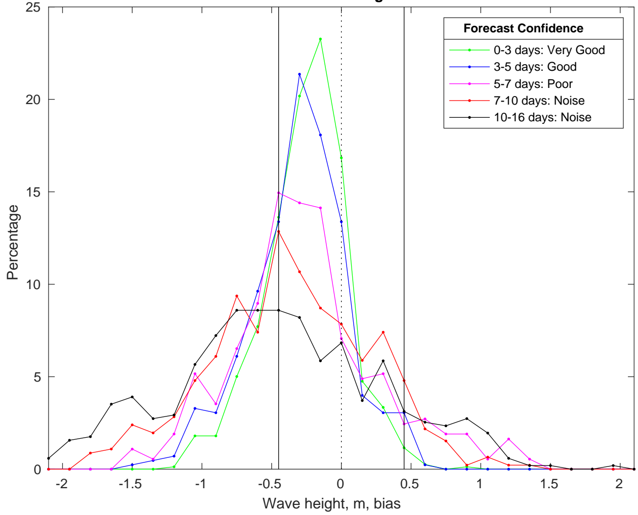
NDBC 46259 vs GFS Waves Bias Histogram: 03-Nov-2025
