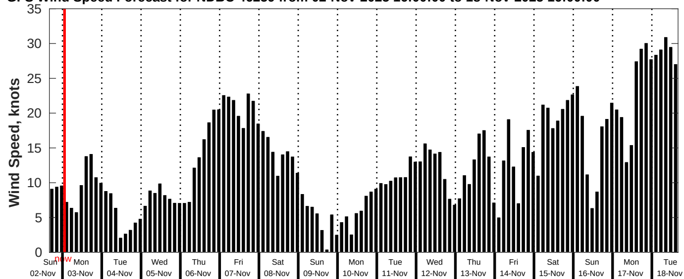
GFS Wind Speed Forecast for NDBC 46259 from 02-Nov-2025 16:00:00 to 18-Nov-2025 16:00:00
