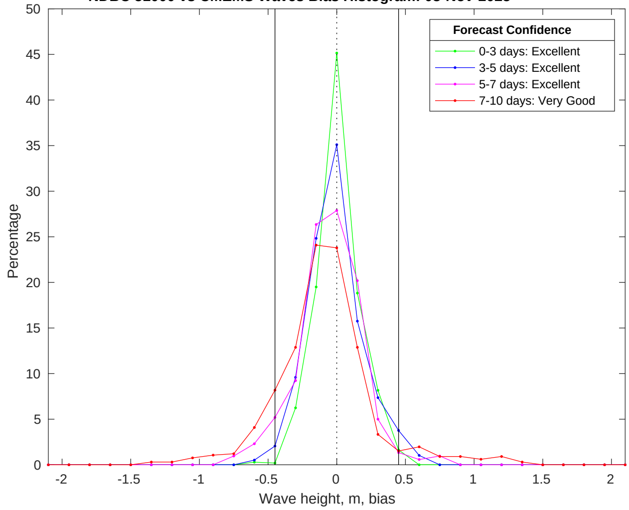
NDBC 51000 vs CMEMS Waves Bias Histogram: 03-Nov-2025
