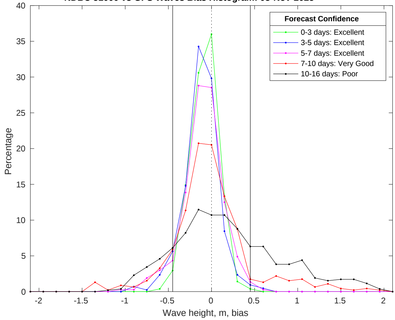
NDBC 51000 vs GFS Waves Bias Histogram: 03-Nov-2025
