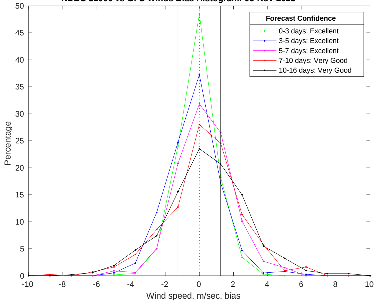
NDBC 51000 vs GFS Winds Bias Histogram: 03-Nov-2025
