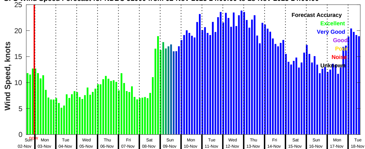
GFS Wind Speed Forecast for NDBC 51000 from 02-Nov-2025 14:00:00 to 18-Nov-2025 14:00:00
