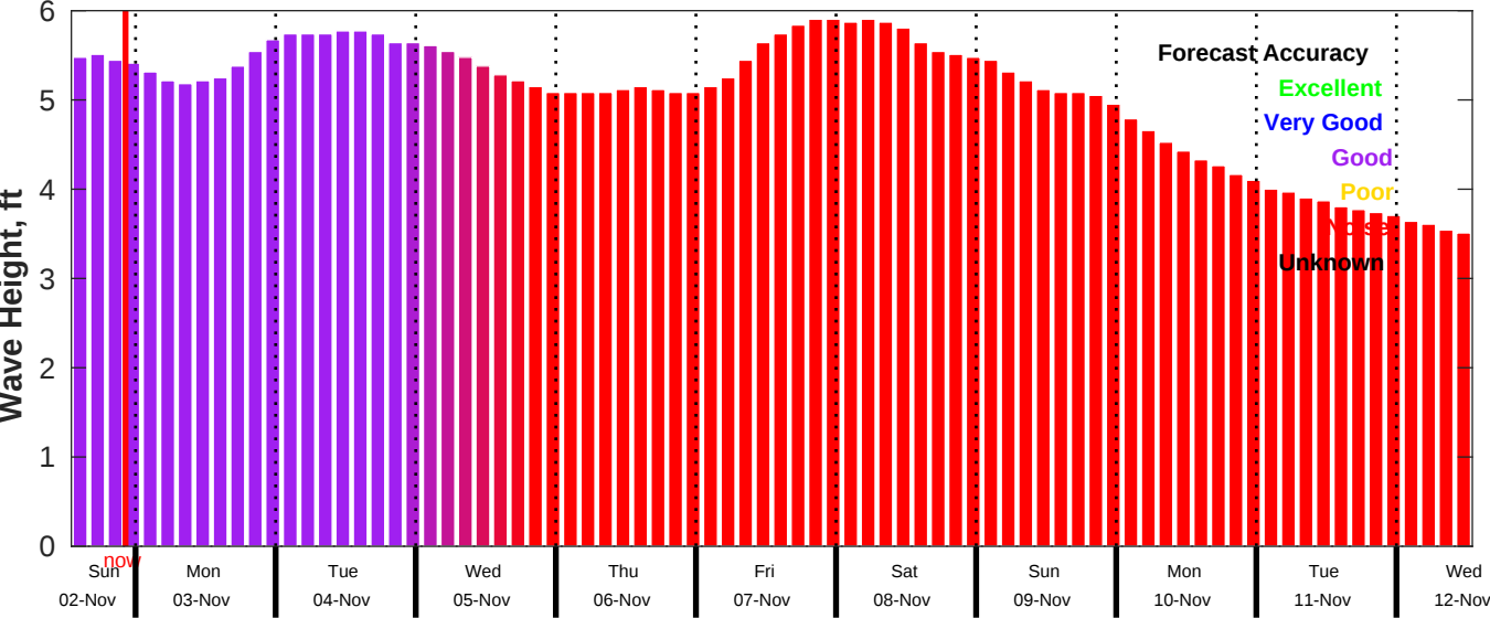
CMEMS Wave Forecast for NDBC 51209 from 02-Nov-2025 13:00:00 to 12-Nov-2025 13:00:00
