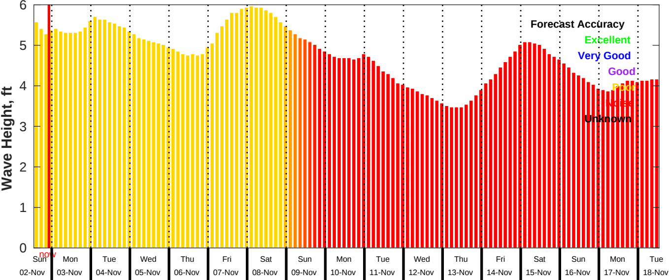
GFS Wave Forecast for NDBC 51209 from 02-Nov-2025 13:00:00 to 18-Nov-2025 13:00:00
