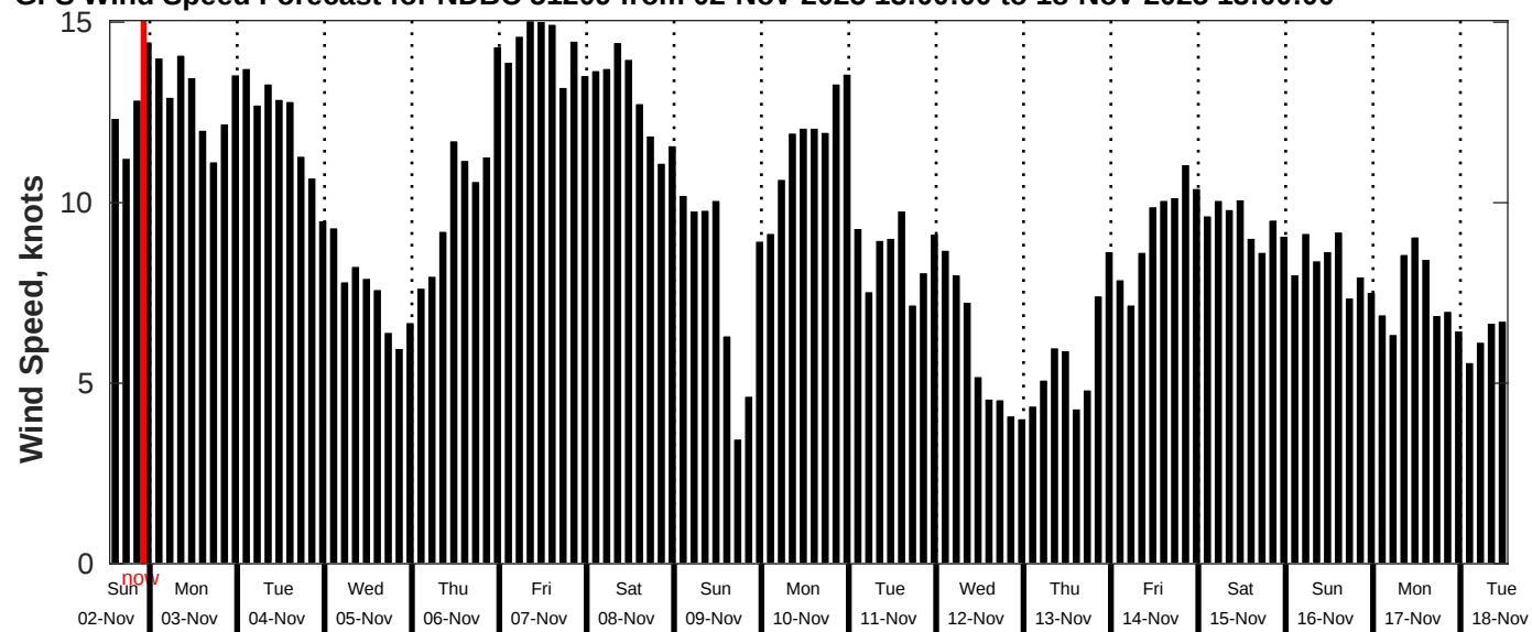
GFS Wind Speed Forecast for NDBC 51209 from 02-Nov-2025 13:00:00 to 18-Nov-2025 13:00:00
