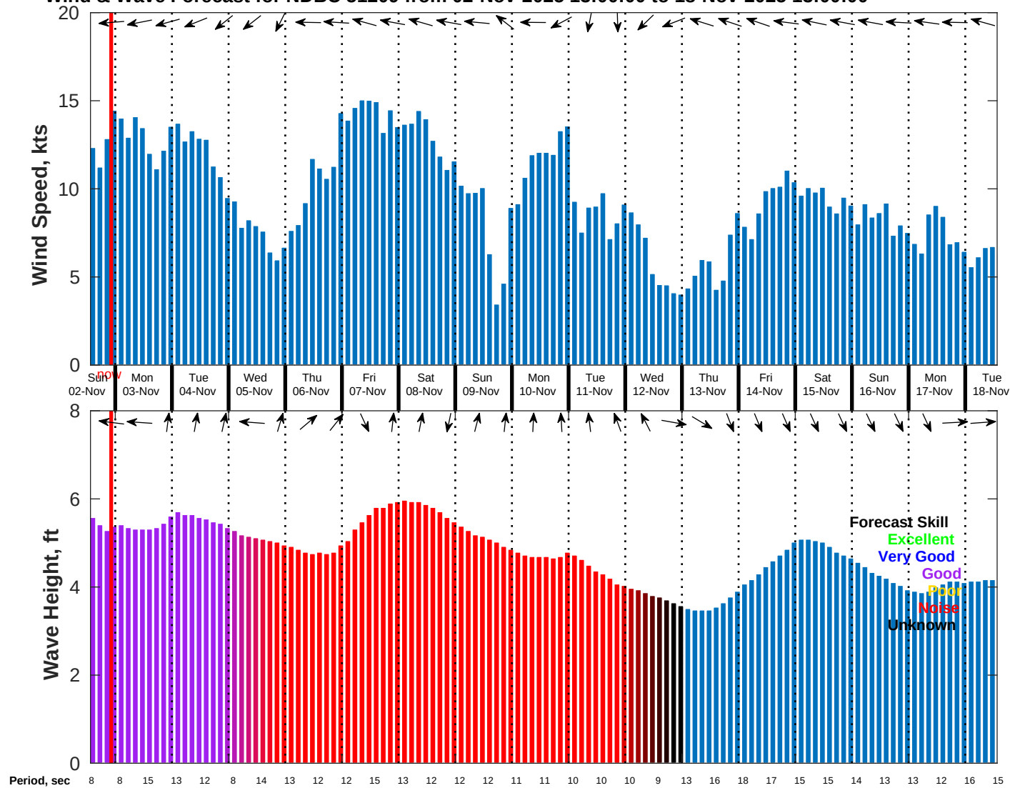
Wind & Wave Forecast for NDBC 51209 from 02-Nov-2025 13:00:00 to 18-Nov-2025 13:00:00
