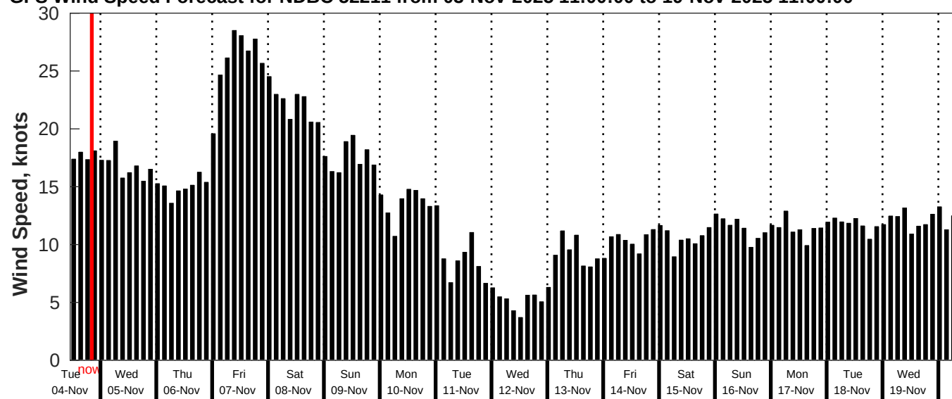
GFS Wind Speed Forecast for NDBC 52211 from 03-Nov-2025 11:00:00 to 19-Nov-2025 11:00:00
