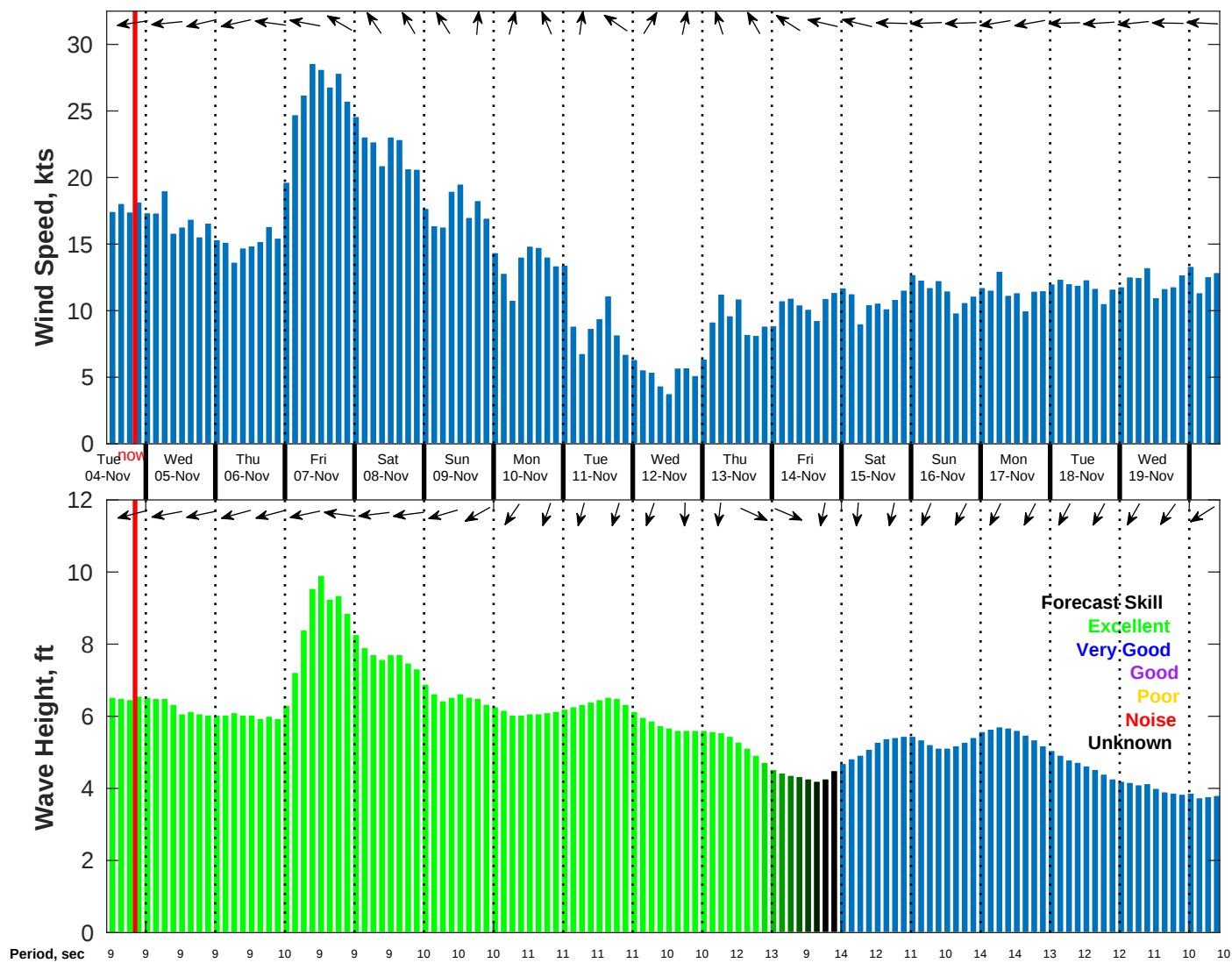
Wind & Wave Forecast for NDBC 52211 from 03-Nov-2025 11:00:00 to 19-Nov-2025 11:00:00
