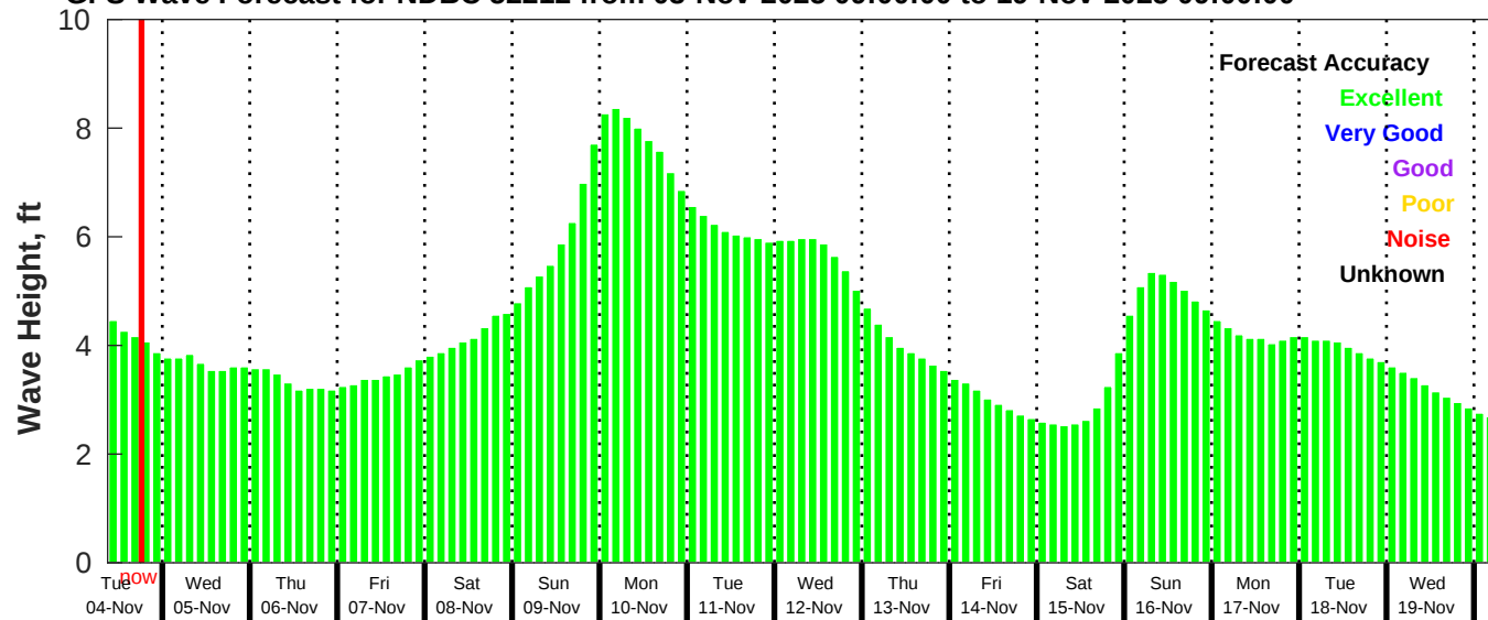
GFS Wave Forecast for NDBC 52212 from 03-Nov-2025 09:00:00 to 19-Nov-2025 09:00:00
