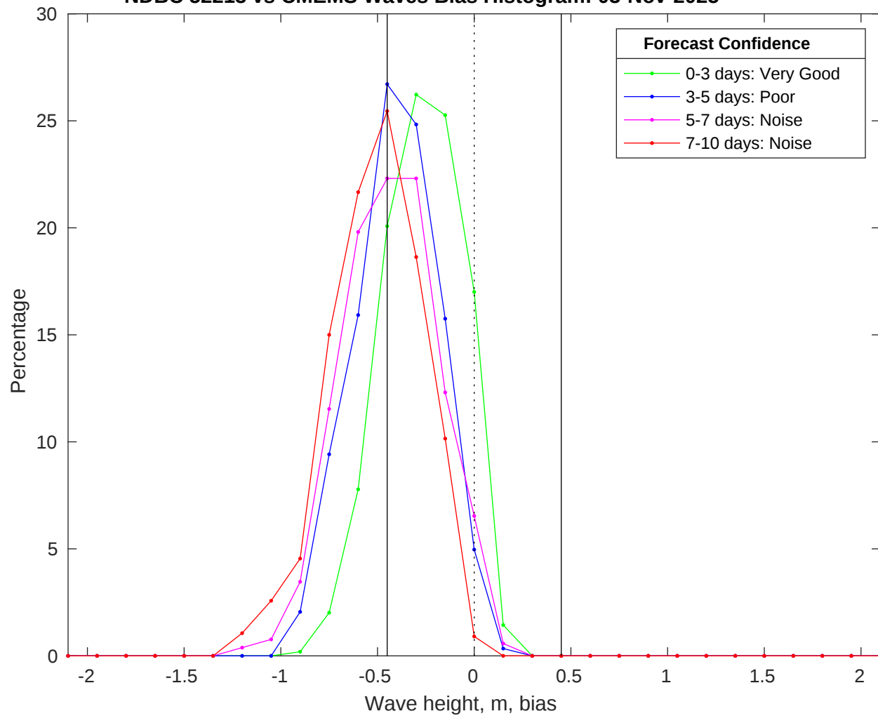
NDBC 52213 vs CMEMS Waves Bias Histogram: 03-Nov-2025
