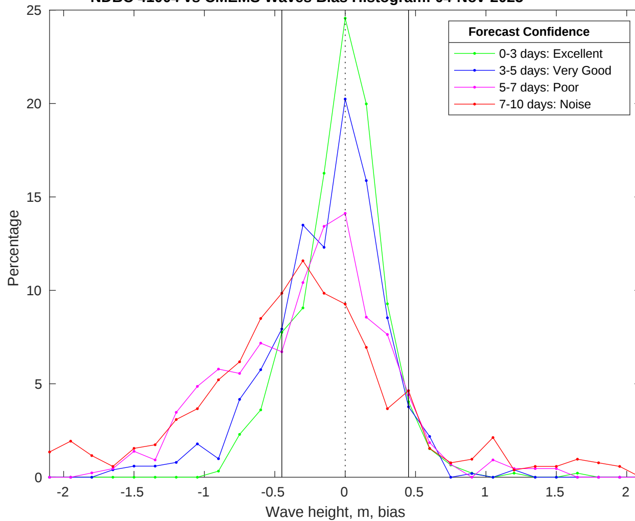
NDBC 41004 vs CMEMS Waves Bias Histogram: 04-Nov-2025
