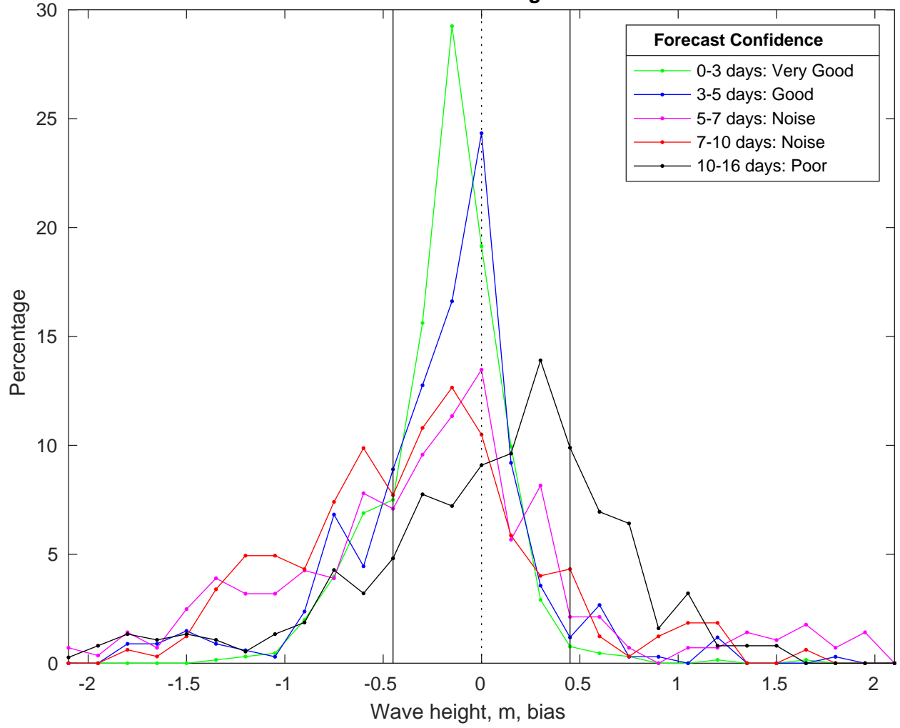
NDBC 41004 vs GFS Waves Bias Histogram: 04-Nov-2025
