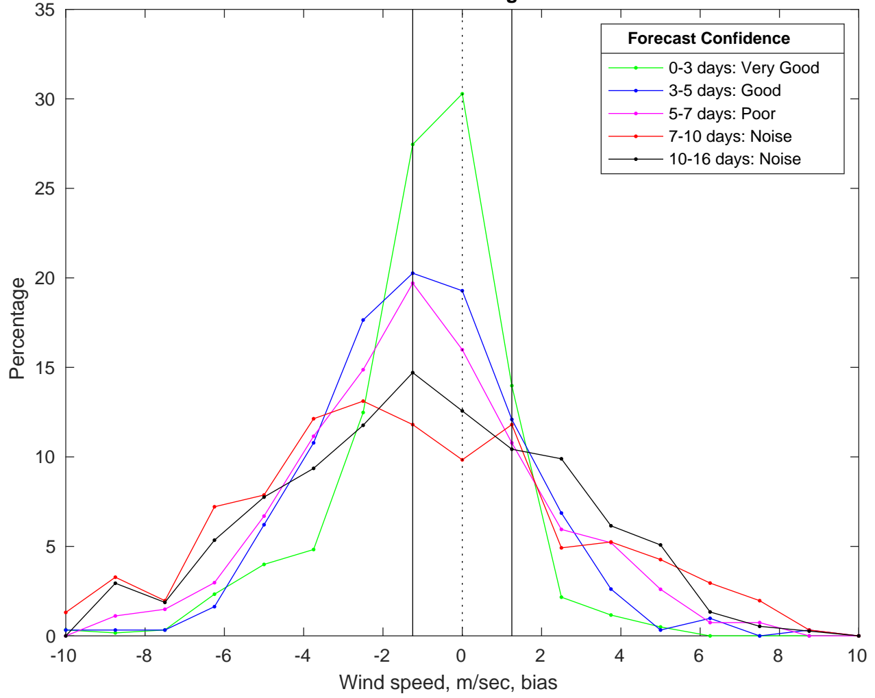
NDBC 41004 vs GFS Winds Bias Histogram: 04-Nov-2025
