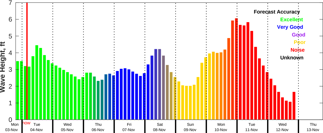
CMEMS Wave Forecast for NDBC 41004 from 03-Nov-2025 19:00:00 to 13-Nov-2025 19:00:00
