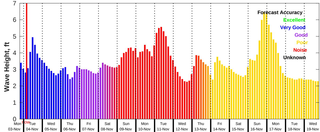
GFS Wave Forecast for NDBC 41004 from 03-Nov-2025 19:00:00 to 19-Nov-2025 19:00:00
