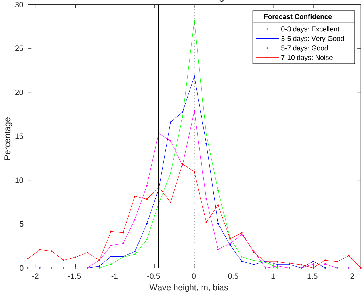
NDBC 41013 vs CMEMS Waves Bias Histogram: 04-Nov-2025
