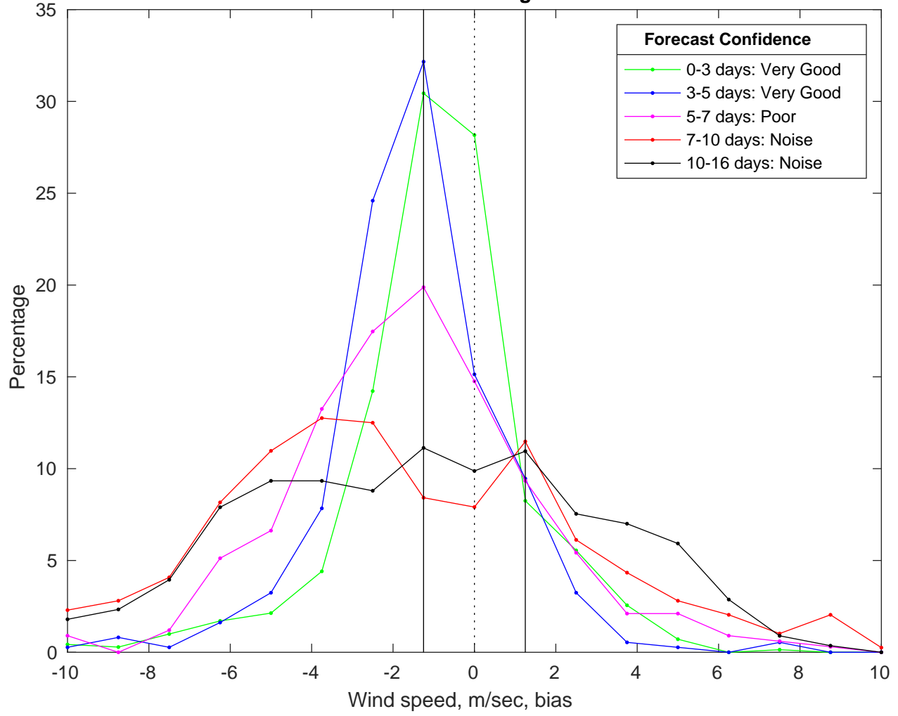
NDBC 41013 vs GFS Winds Bias Histogram: 04-Nov-2025
