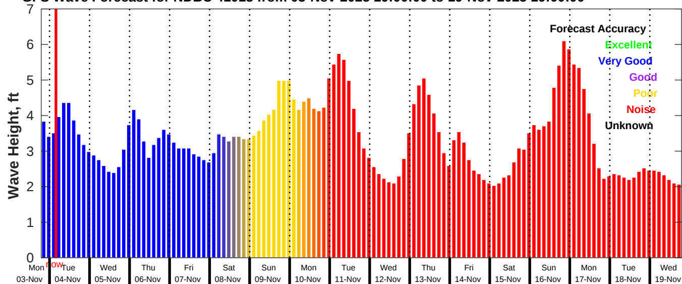
GFS Wave Forecast for NDBC 41013 from 03-Nov-2025 19:00:00 to 19-Nov-2025 19:00:00
