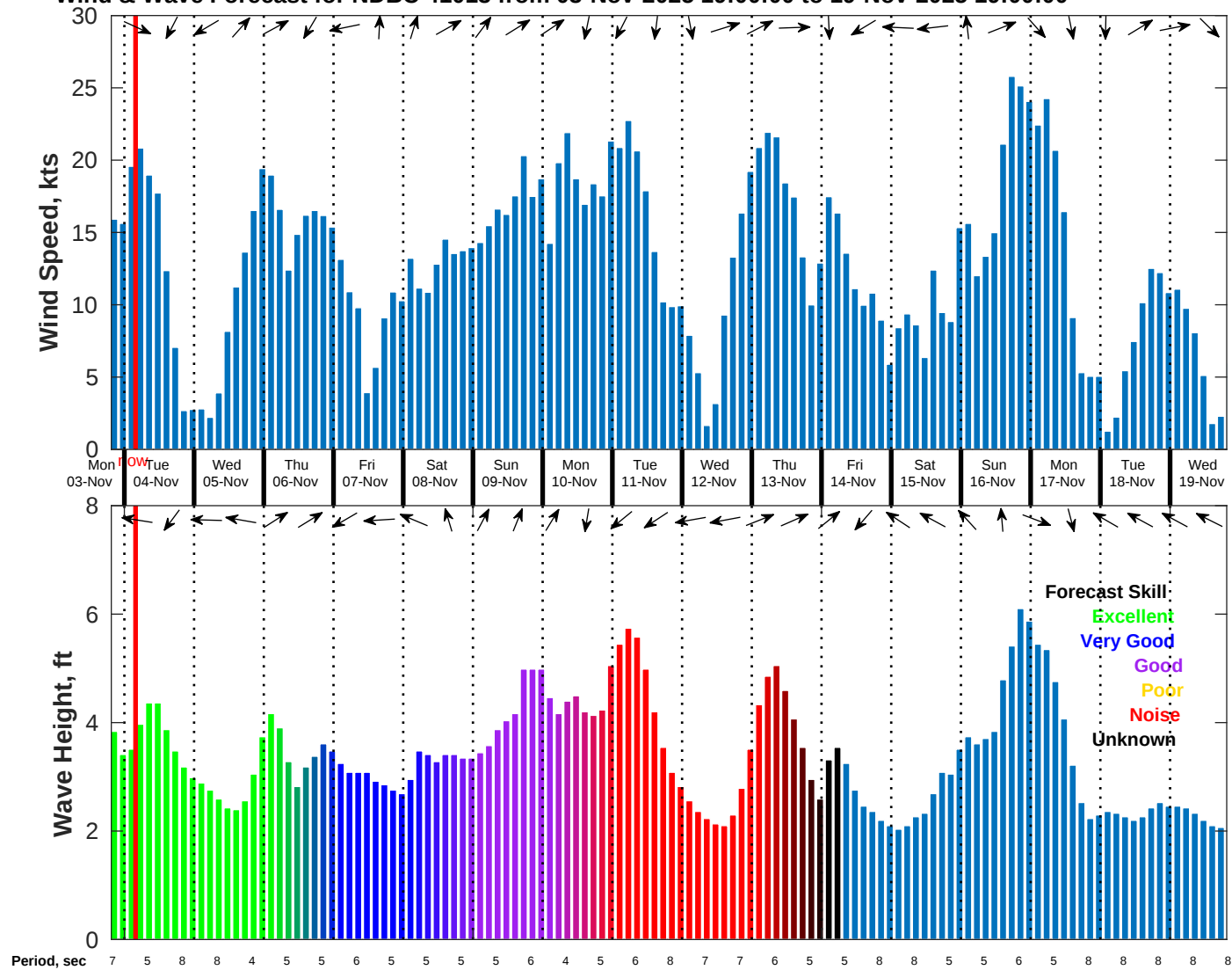
Wind & Wave Forecast for NDBC 41013 from 03-Nov-2025 19:00:00 to 19-Nov-2025 19:00:00
