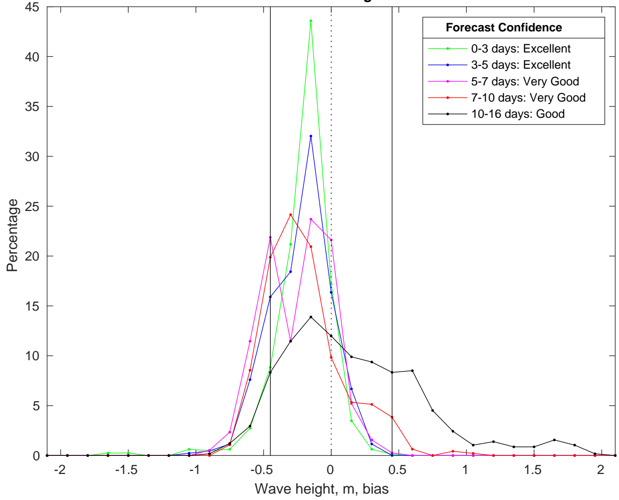
NDBC 41040 vs GFS Waves Bias Histogram: 04-Nov-2025
