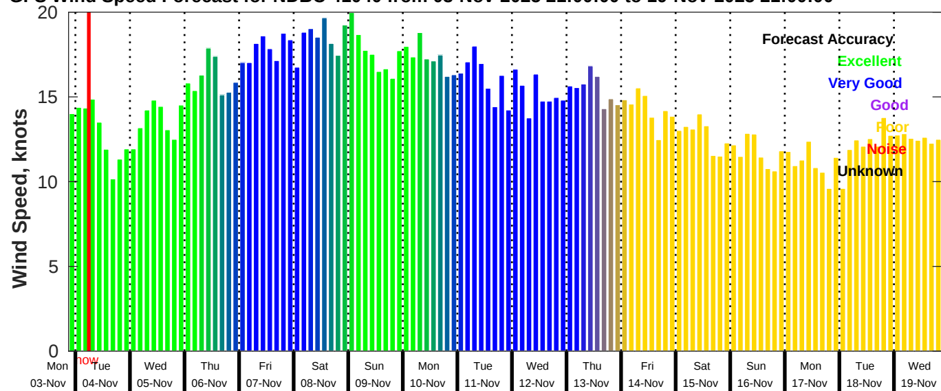
GFS Wind Speed Forecast for NDBC 41040 from 03-Nov-2025 21:00:00 to 19-Nov-2025 21:00:00
