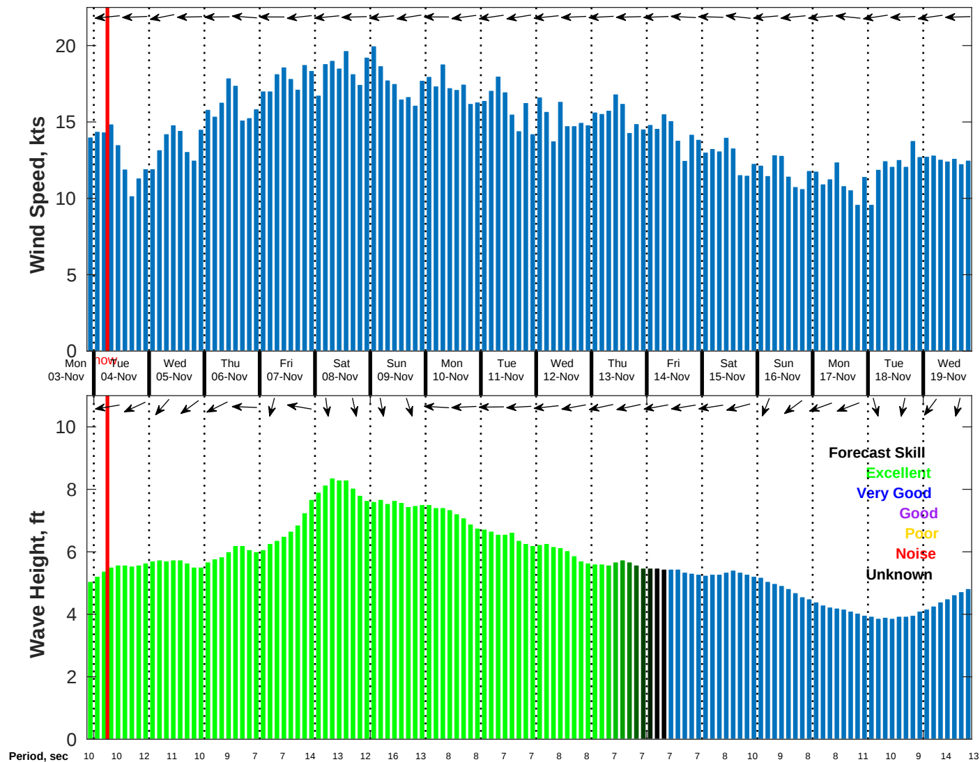
Wind & Wave Forecast for NDBC 41040 from 03-Nov-2025 21:00:00 to 19-Nov-2025 21:00:00
