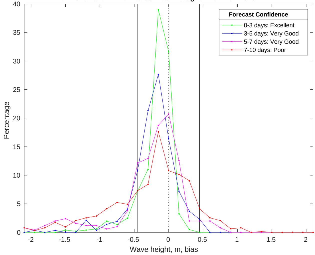
NDBC 42019 vs CMEMS Waves Bias Histogram: 04-Nov-2025
