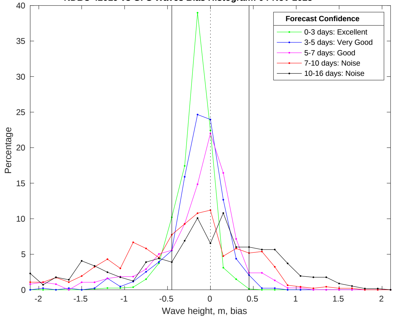
NDBC 42019 vs GFS Waves Bias Histogram: 04-Nov-2025
