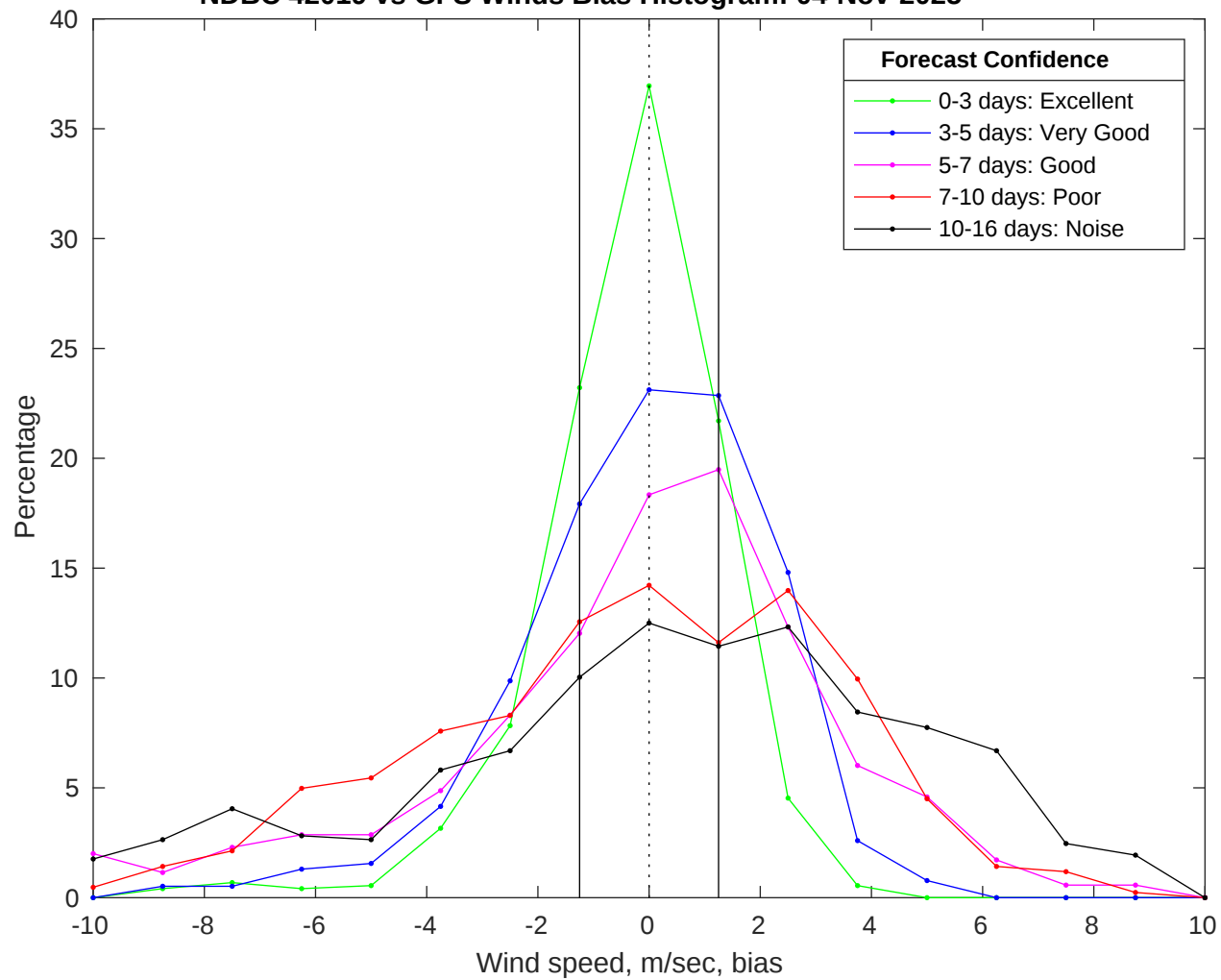
NDBC 42019 vs GFS Winds Bias Histogram: 04-Nov-2025
