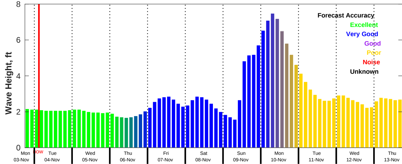
CMEMS Wave Forecast for NDBC 42019 from 03-Nov-2025 18:00:00 to 13-Nov-2025 18:00:00
