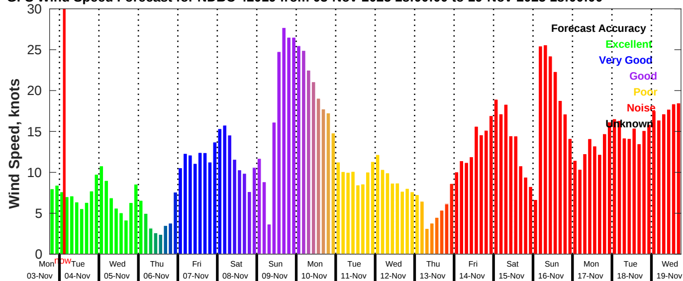
GFS Wind Speed Forecast for NDBC 42019 from 03-Nov-2025 18:00:00 to 19-Nov-2025 18:00:00
