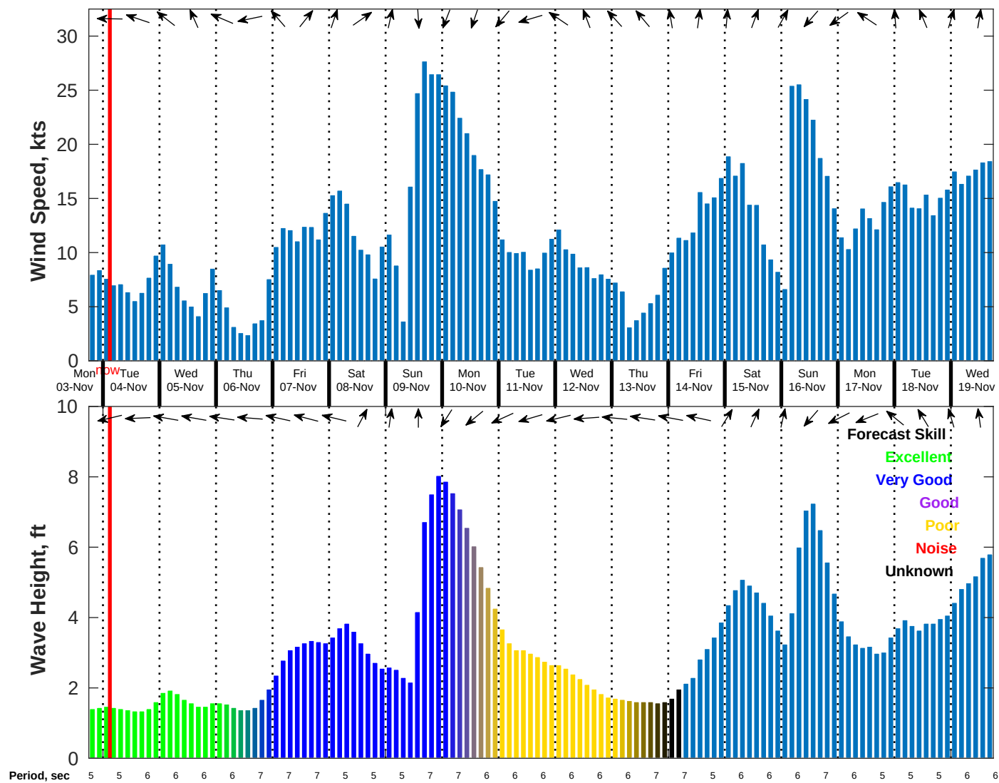
Wind & Wave Forecast for NDBC 42019 from 03-Nov-2025 18:00:00 to 19-Nov-2025 18:00:00
