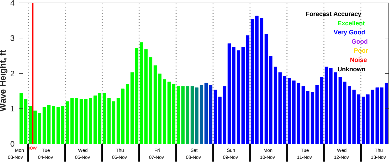
CMEMS Wave Forecast for NDBC 42035 from 03-Nov-2025 18:00:00 to 13-Nov-2025 18:00:00
